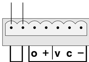
Thermistor Anschlüsse
